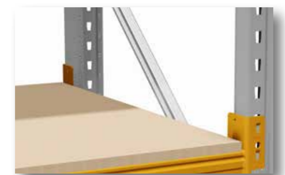
Board sits on top of the Box Beam profile and is secured by retainers.
