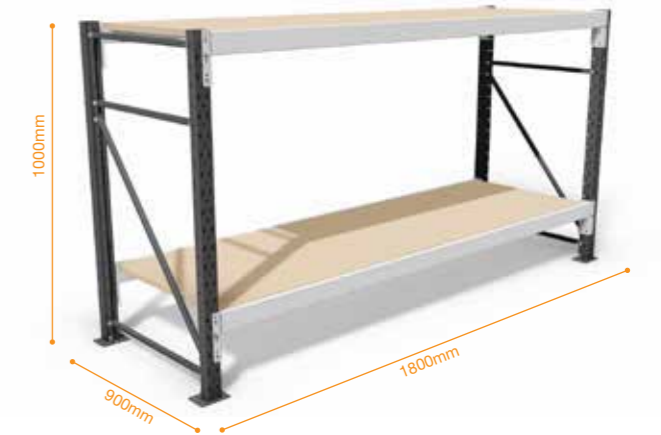
Ultima Longspan 2 workbench with particle board work surface and bottom shelf.
